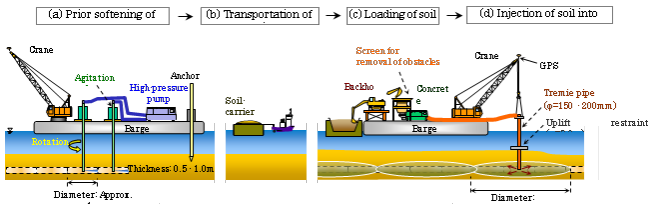
Sketch of the drag anchor installation and its FE model (After Liu and Zhao, 2014)
