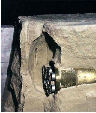
Unsupported cavity (After König et al., 2014)
