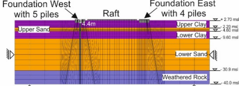
Cross section through the finite element mesh
