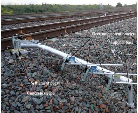
2. Track Displacement Monitoring (Indraratna et al , 2014)
