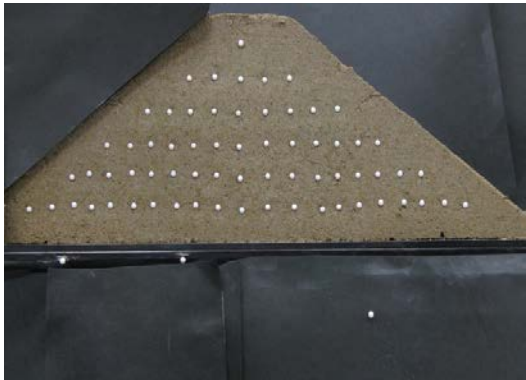
Large Model with guage points for shear and volumetric strain measurement (after Miyanaga, et al , 2013)
