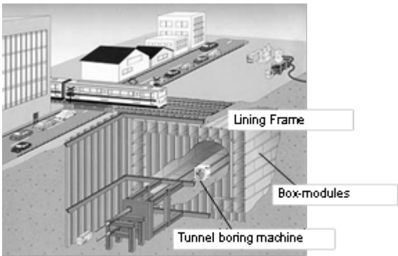
Box Jacking Tunnelling (after Komiya and Nakayama, 2013)
