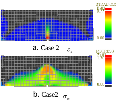
Simulation in Cement Treated Soil
