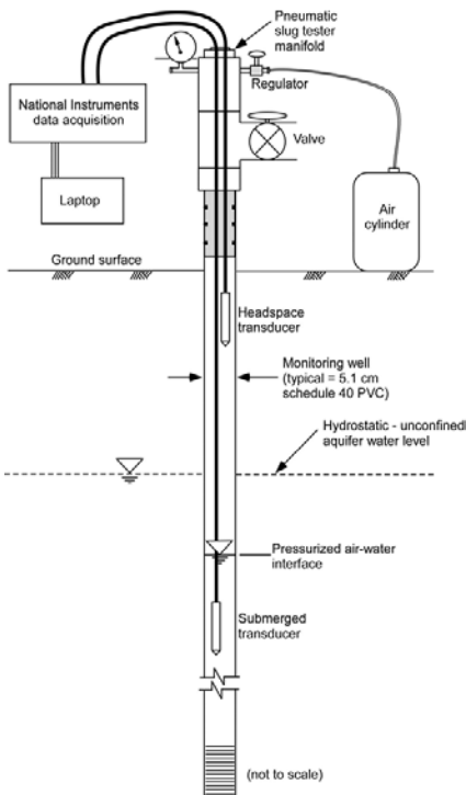
Hydraulic Conductivity Test (After DeGroot et al, 2012; Dunaj et al. 2006)
