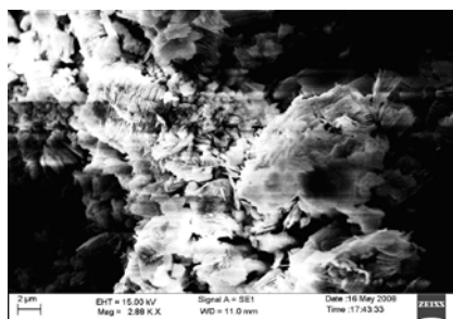
SEM Image of Residual Soil of Singapore Bukit Timah Granite, (after Meng & Chu, 2011)
