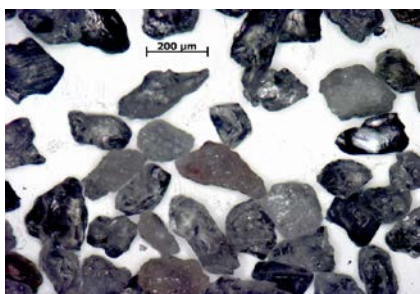
50 x SEM Image of a Sand (after Georgiannou, 2011)
