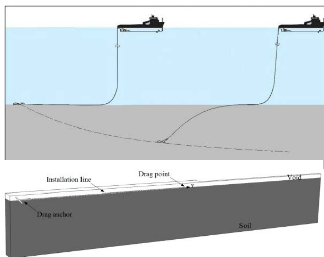
Sketch of the drag anchor installation and its FE model (After Liu and Zhao, 2014)
