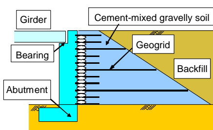
a. GRS bridge abutment
