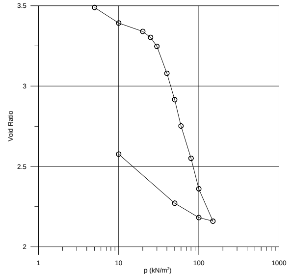
Fig. 1 Consolidation process of clay sample
