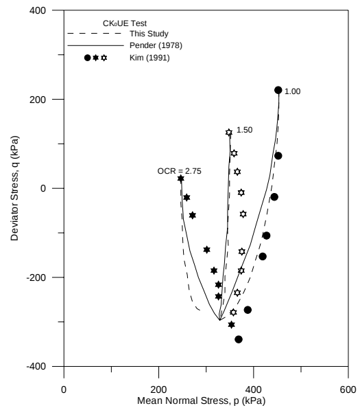
Fig. 17 Undrained stress paths compared with the model predictions (CK 0 UE test)
