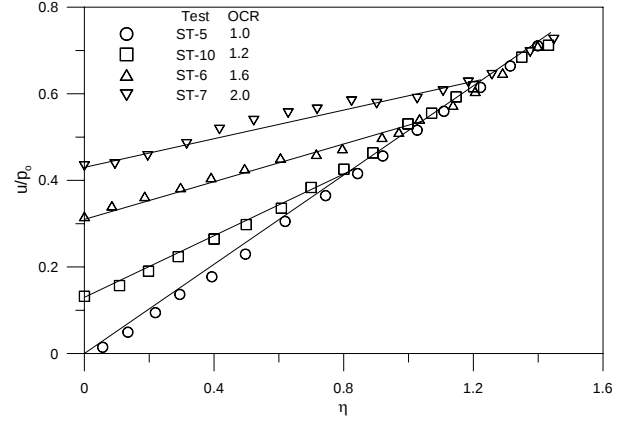
Fig. 6 Shifted (u/p_0, \eta) plots for over-consolidated samples
