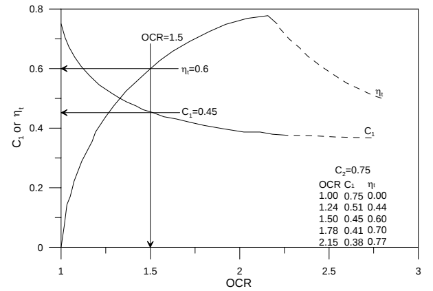
Fig. 8 OCR - C_1 - \eta relationship from CID samples
