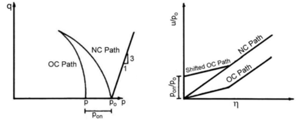
Fig. 7 Shifting of (u/p_0, \eta) plot for overconsolidated samples
