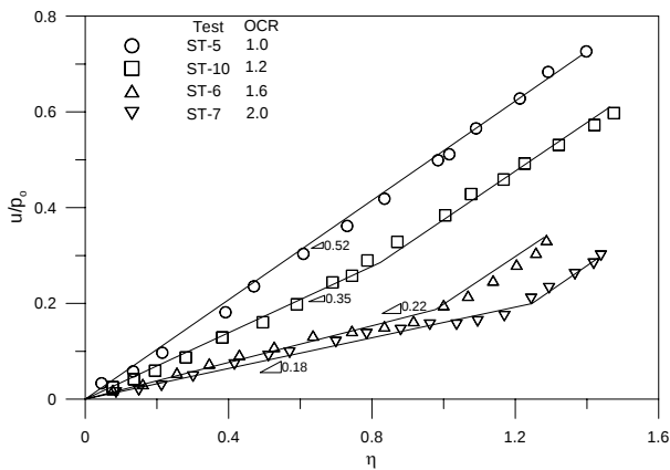
Fig. 5 (u/p_0, \eta) plots for over-consolidated samples under monotonic loading
