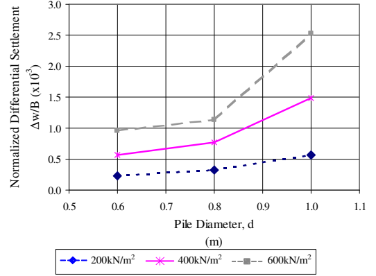
Figure 7. Normalized differential settlement vs. pile diameter
