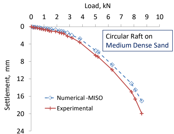
Figure 8 Comparison of load-settlement behaviour in numerical analyses and in model test
