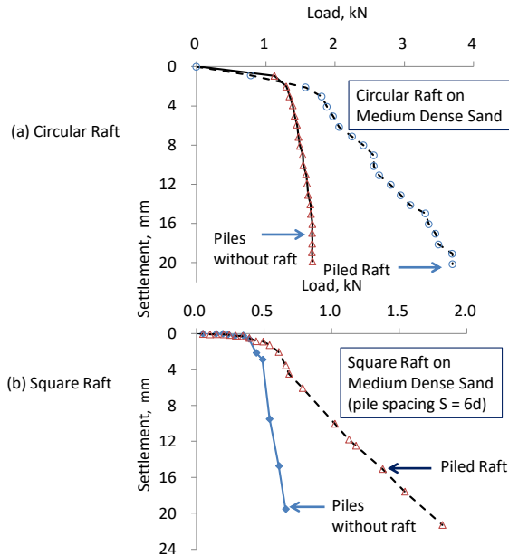
Figure 5 Settlements of piles with and without raft
