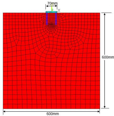
Figure 9 Finite element mesh used for rectangular pile raft in plane strain analysis using ANSYS
