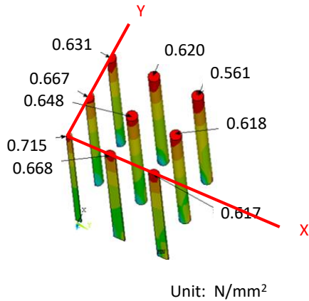
Figure 17 Stresses at tips of piles for 8.7kN load
