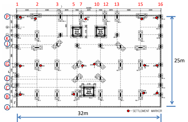
Figure 21 Plan and layout of piles
