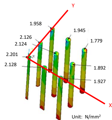
Figure 16 Stresses on pile heads for 8.70kN load
