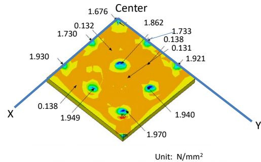
Figure 15 Vertical stress under the square piled raft with piles for the load of 8.7kN
