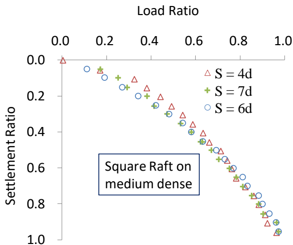
Figure 6 Settlements of square piled raft with different pile spacings
