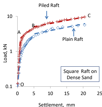
Figure 3 Settlements of square raft, with and without piles, resting on dense sand
