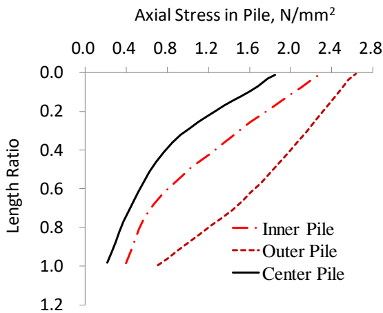
Figure 18 Variation of axial stress along the shaft of typical piles under the circular piled raft for a load of 8.10kN
