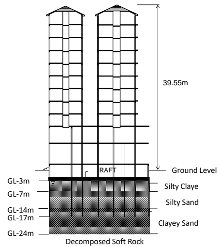
Figure 20 Elevation of the case analyzed
