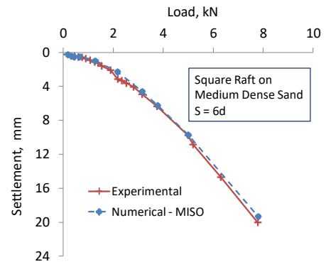
Figure 14 Comparison of load -settlement response between ANSYS and test data for square piled raft with 6d pile spacing
