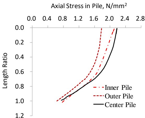
Figure 19 Variation of axial stress along the shaft of typical piles under the square piled raft for a load of 8.10kN
