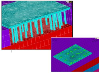
Figure 22 Finite Element Simulation and Meshing of Piled Raft
