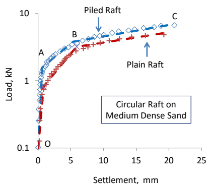
Figure 2 Settlements of circular raft, with and without piles, resting on medium dense sand
