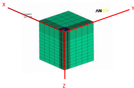
Figure 12 Finite element mesh of a quadrant of the system adopted for square piled raft in ANSYS analysis
