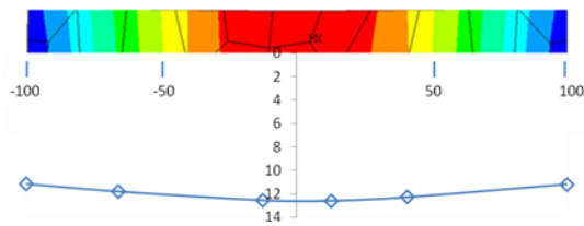
Figure 10 Settlement of piled raft at the load of 1.55 kN
