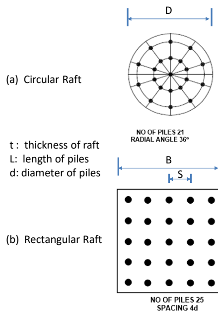
Figure 1 Layout of piles supporting the rafts
