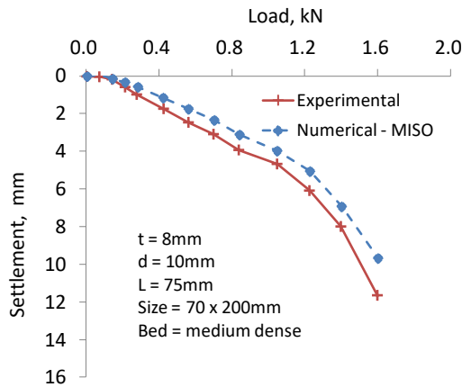
Figure 11 Comparison of load-settlement response between ANSYS and test data for rectangular piled raft
