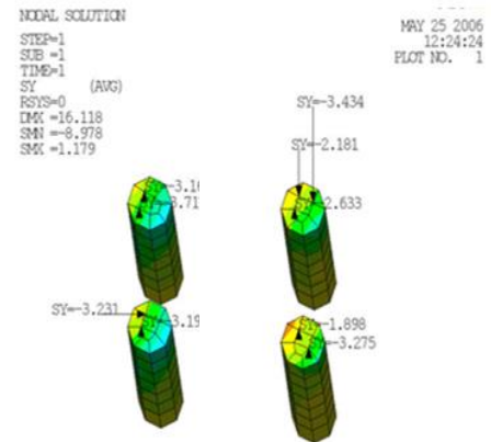
Figure 25 Typical head stress values
