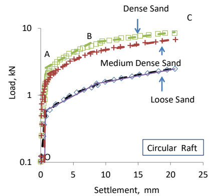
Figure 4 Effects of foundation soils on the settlements of piled rafts
