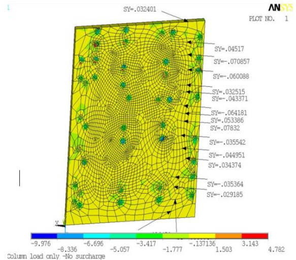
Figure 24 Distribution of stresses at raft-pile interface
