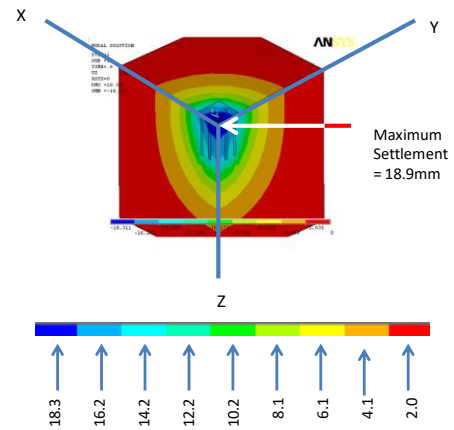
Figure 13 Settlement contour for the load of 8.70kN (settlement 18.90mm)
