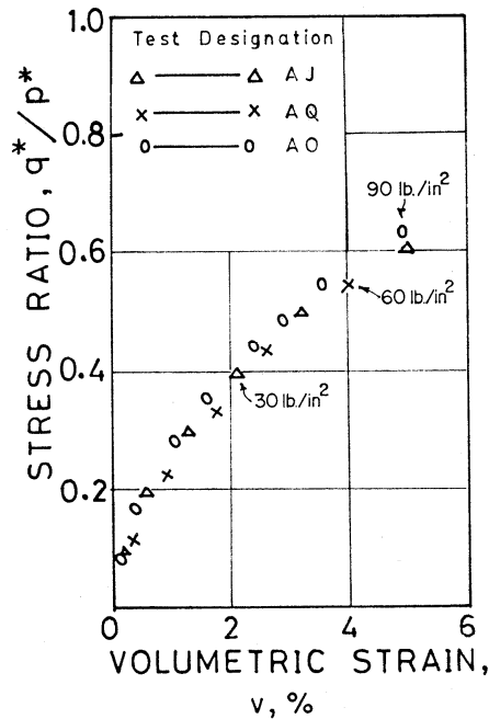
Fig. 23. The (q^*/p^*, v^*) characteristics of Specimens AJ, AQ and AO prepared under an initial one-dimensional consolidation stress of 22 lb/in 2 and sheared under p -constant condition from isotropic stresses of 30, 60 and 90 lb/in 2 respectively.
