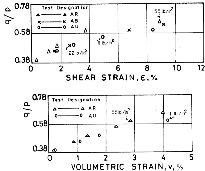
Fig. 4. The (q/p, \epsilon) and (q/p, v) characteristics beyond a stress ratio of 0.375.
