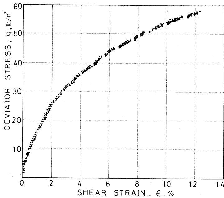
Fig. 16. The (q, \epsilon) relationship for Specimen Z sheared under small load increments.
