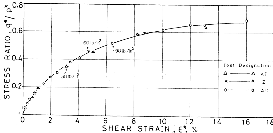
Fig. 26. The (q^*/p^*, \epsilon^*) characteristics of Specimens AF, Z and AD.
