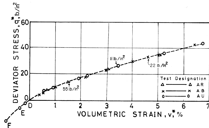
Fig. 8. The (q^*, v^*) characteristics of Specimens AR, AB and AU prepared under different initial one-dimensional stresses and sheared under fully drained conditions from an isotropic stress of 60 lb/in 2 with constant cell pressure.
