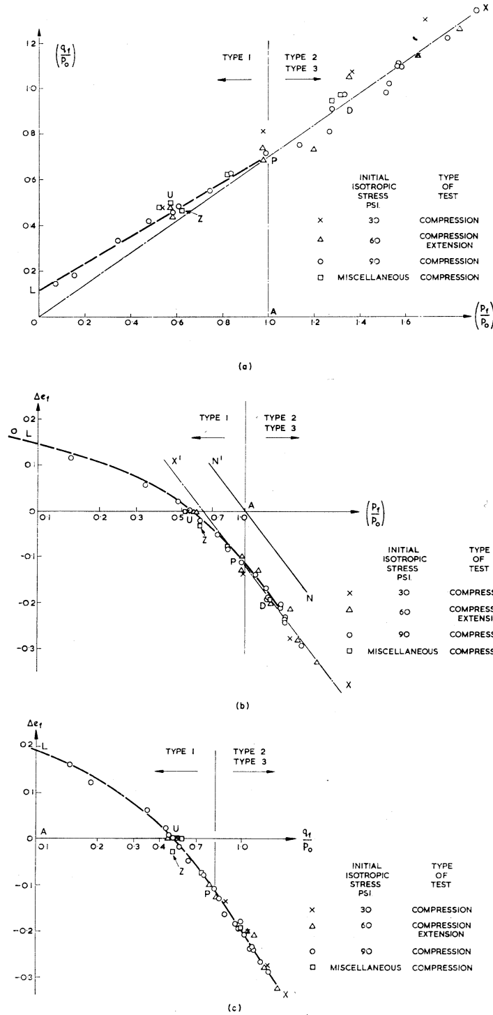
Fig. 7. The (q_f/p_o, p_f/p_o) , (\Delta e_f, \ln(p_f/p_o)) and (\Delta e_f, \ln(q_f/p_o)) characteristics of all specimens sheared along Type 1, Type 2 and Type 3 test paths.
