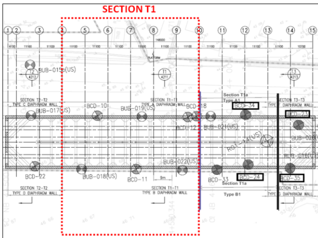
Figure 2A Merdeka Station boreholes layout
