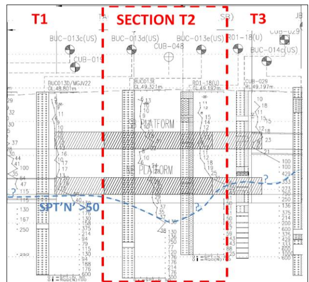
Figure 3B Bukit Bintang Simplified Subsurface profile
