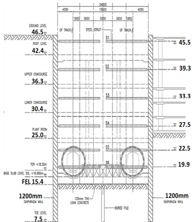
Figure 4A Merdeka Station Cross Section T2
