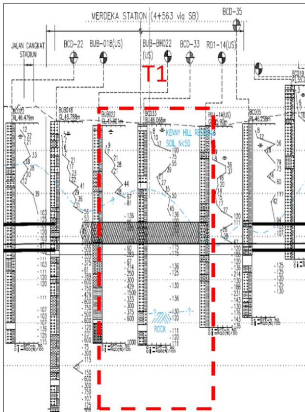
Figure 2B Merdeka Station simplified subsurface profile
