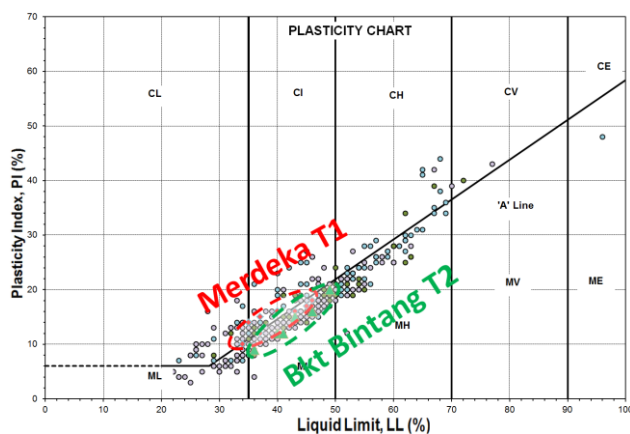
Figure 3D Plasticity Chart of Kenny Hill Soils
