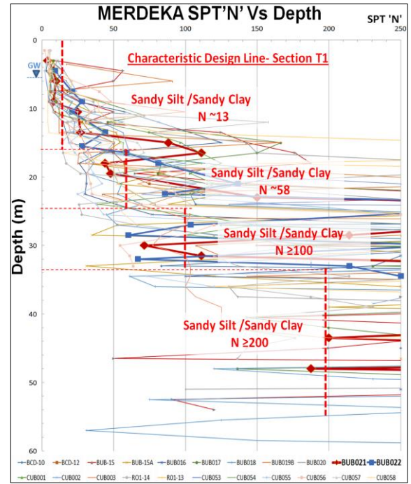
Figure 2C Merdeka Station Characteristic Design Line for D-Wall Section T1
