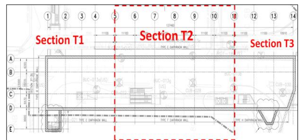
Figure 3A Bukit Bintang Station Borehole layout
