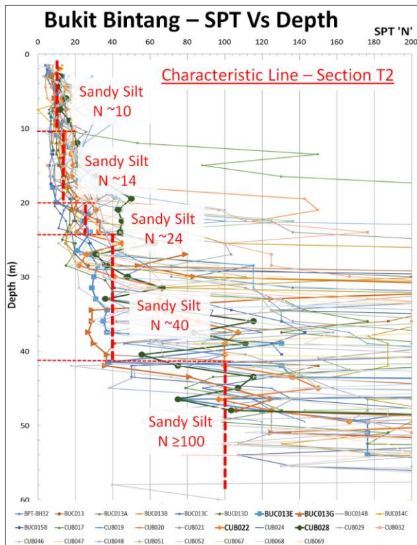
Figure 3C Bukit Bintang Station Characteristic Design Line for D-Wall Section T2
