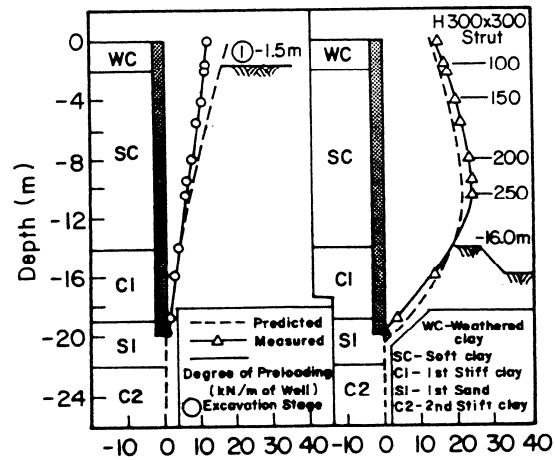
Fig. 14 Diaphragm wall deflection profile at site D
