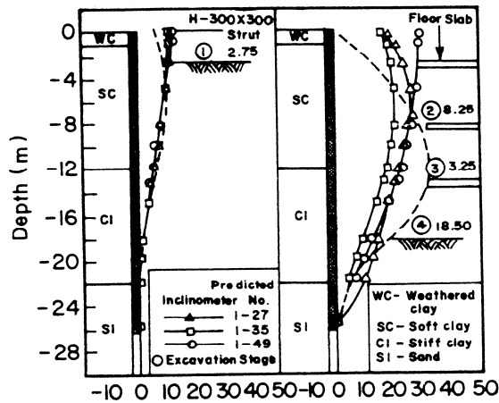
Fig. 13 Diaphragm wall deflection profile at site C
