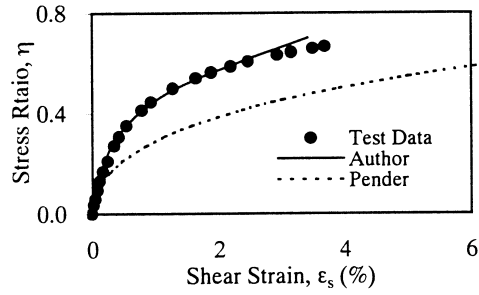
Fig. 7 (\eta, \epsilon_s) Plot for CID test compared with model prediction (OCR=2.15)
