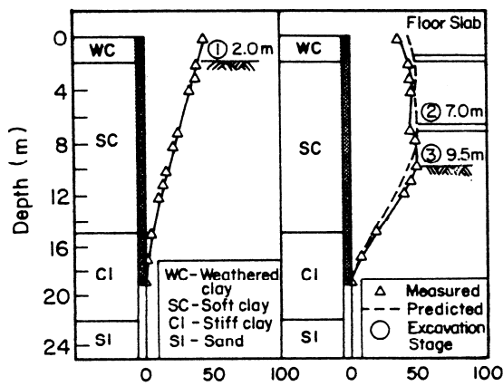
Fig. 11 Diaphragm wall deflection profile at site A
