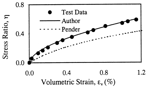
Fig. 6 (\eta, \epsilon_v) Plot for CID test compared with model prediction (OCR=2.15)
