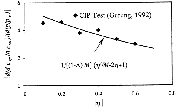
Fig. 3 Variation of (d\epsilon_v^p / d\epsilon_s^p) / (p / p_e) versus the stress ratio within SBS
