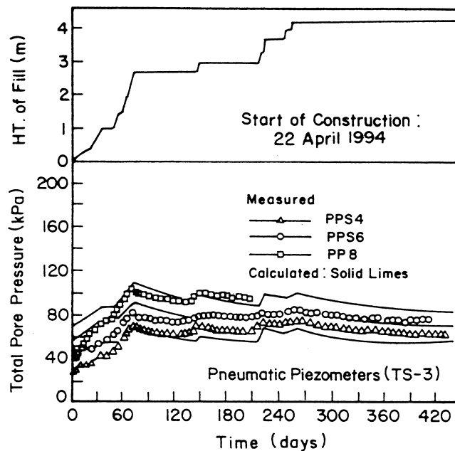
Fig. 10 Computed pore pressure from FEM and measured values- TS3
