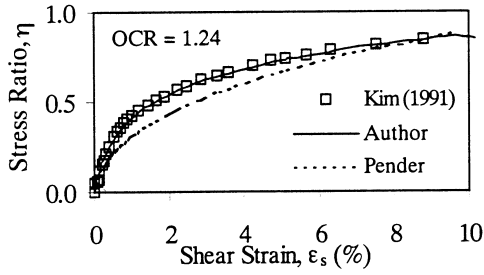
Fig. 4 (\eta, \epsilon_s) Plot for CIU sample compared with model prediction
