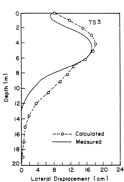
Fig. 9 Comparison of computed FEM and measured lateral deformations
