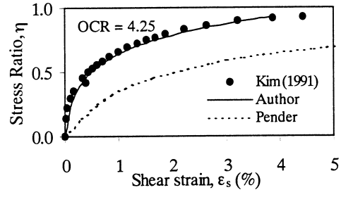
Fig. 5 (\eta, \epsilon_s) Plot for CIU sample compared with model prediction
