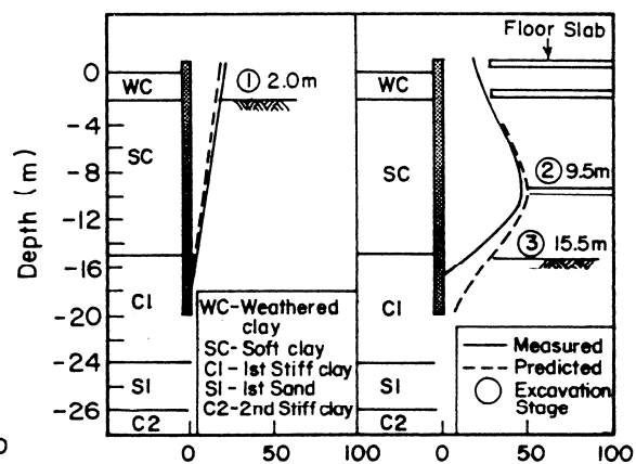
Fig. 12 Diaphragm wall deflection profile at site B
