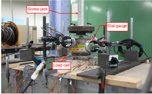
Figure 4 Experiment setup with measuring instruments in vertical load tests
