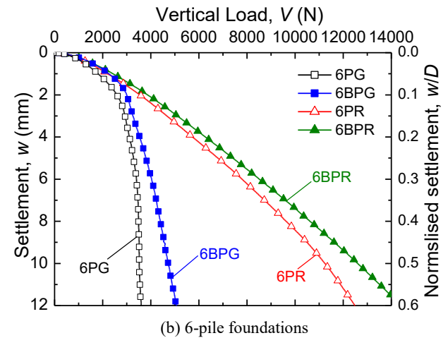
Figure 9 Load-settlement curves of the foundation models
