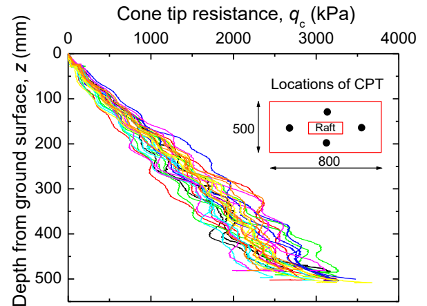
Figure 7 The results of Cone Penetration Tests
