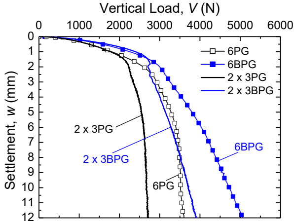
Figure 16 Load-settlement curves for 6PG, 6BPG, 2x3PG and 2x3BPG
