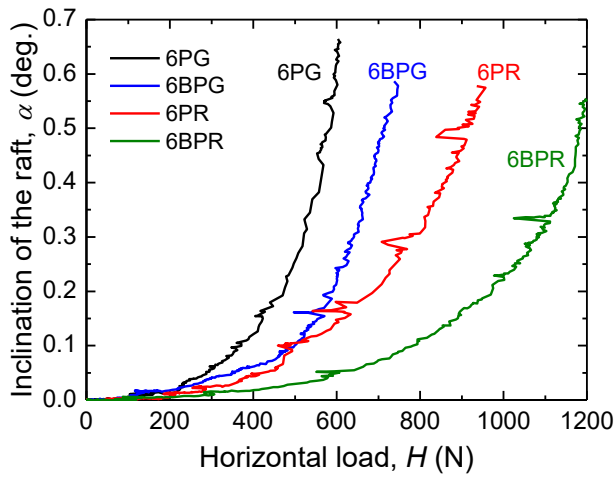
Figure 21 Inclination of the raft vs. horizontal load during the initial loading stage for 6PG, 6BPG, 6PR and 6BPR
