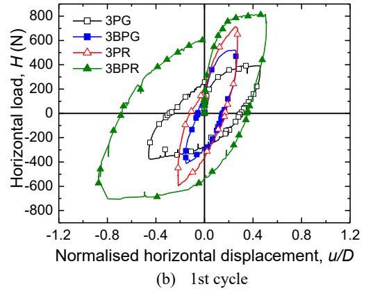
Figure 18 Horizontal load-normalised horizontal displacement curves for 3PG, 3BPG, 3PR and 3BPR
