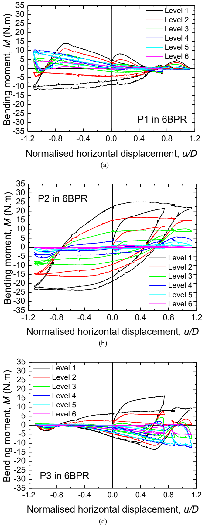
Figure 28 Bending moments of piles for 6BPR (in HLT)
