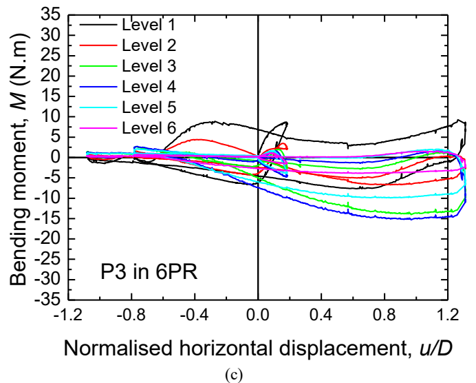
Figure 27 Bending moments of piles for 6PR (in HLT)
