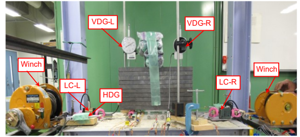
Figure 6 Experiment setup with measuring instruments in combination load tests
