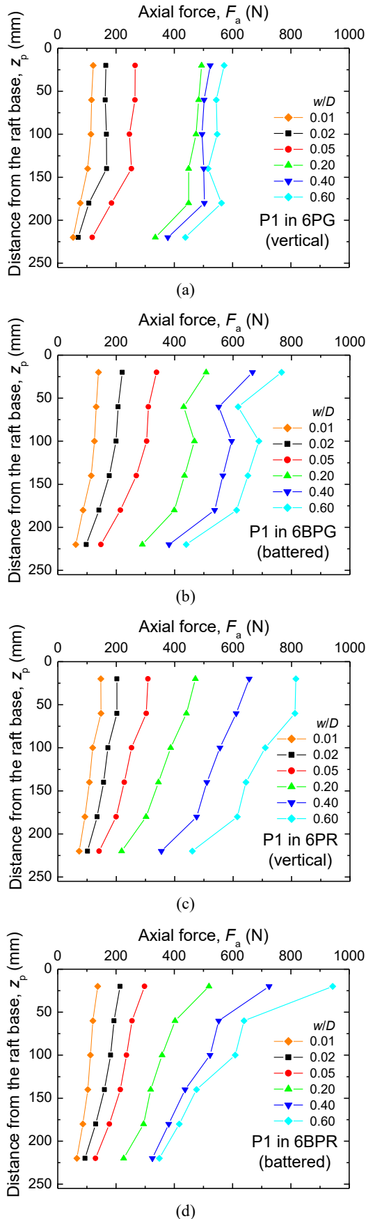
Figure 13 Axial force distributions along pile shaft of P1 in the cases of 6PG, 6BPG, 6PR and 6BPR
