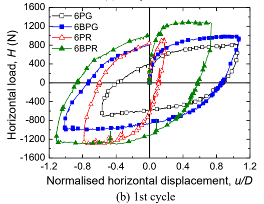
Figure 19 Horizontal load-normalised horizontal displacement curves for 6PG, 6BPG, 6PR and 6BPR
