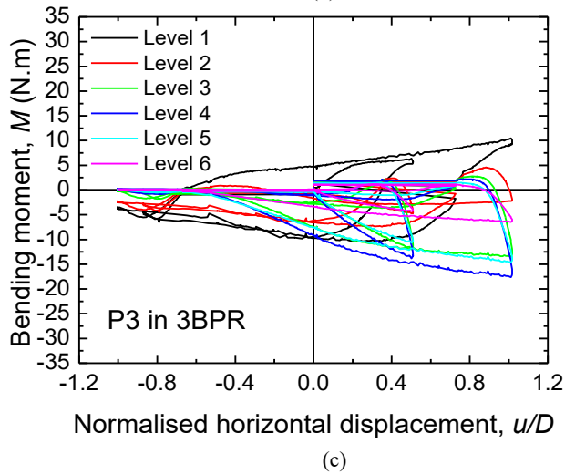
Figure 26 Bending moments of piles for 3BPR (in HLT)
