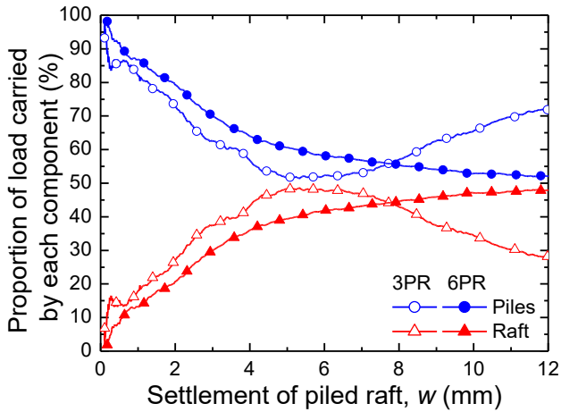
Figure 11 Proportions of vertical load carried by the pile component and the raft component in the cases of 3PR and 6PR
