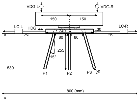
Figure 5 Schematic illustration of a combination load test
