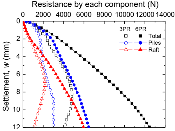
Figure 10 Load-settlement curves in cases of 3PR and 6PR
