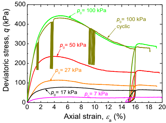
(a) Axial strain \varepsilon_a versus deviatoric stress q
