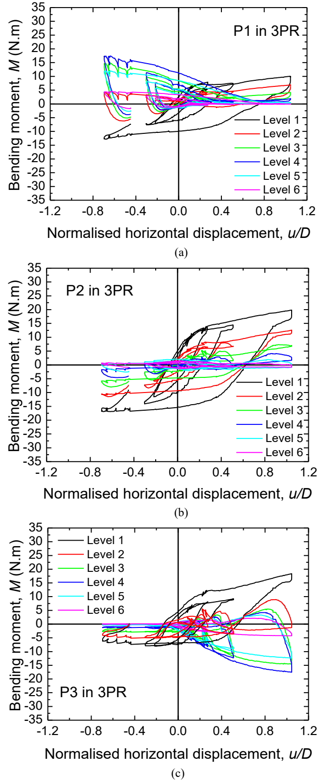
Figure 25 Bending moments of piles for 3PR (in HLT)
