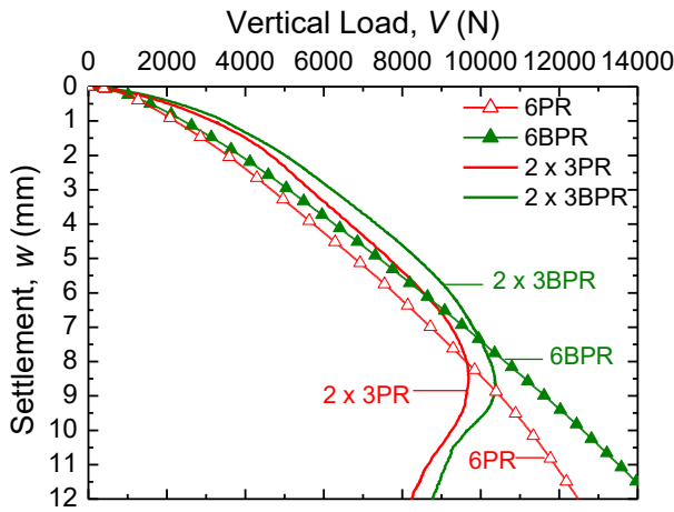
Figure 17 Load-settlement curves for 6PR, 6BPR, 2x3PR and 2x3BPR
