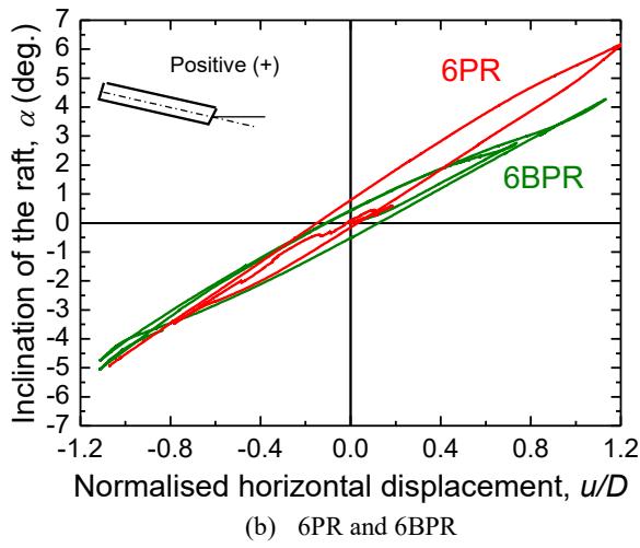
Figure 20 Inclination of the raft during cyclic horizontal load
