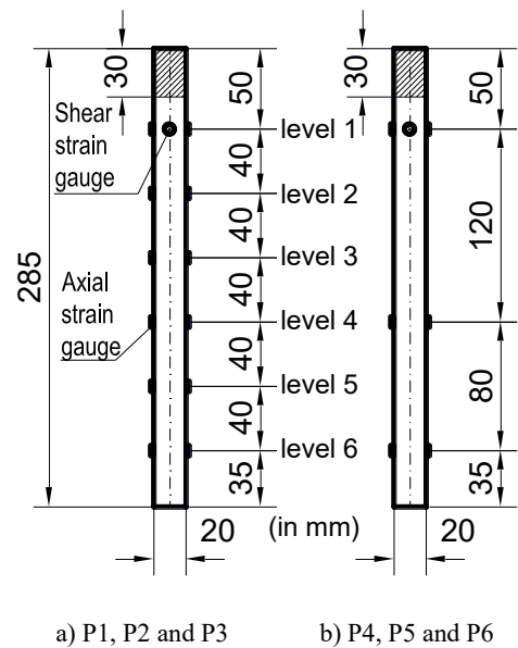
Figure 2 Model piles with strain gauge instrumentation
