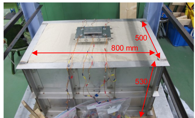
Figure 3 Dimensions of the soil box
