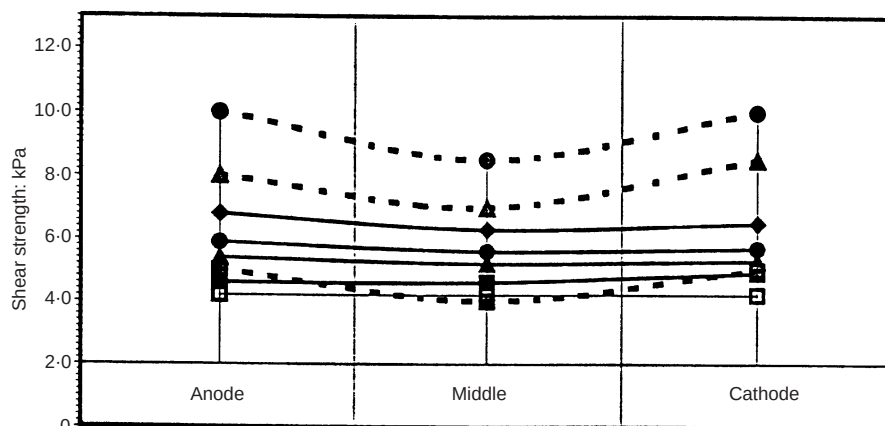
Fig. 11. Shear strength increase due to electro-osmotic consolidation with PVDs using small cylinder apparatus
