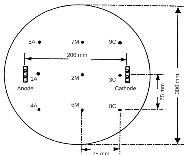
Fig. 7. Shear strength test location points for the small cylinder electro-osmotic cell
