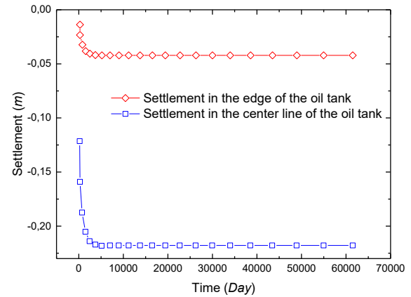
Figure 4 Evolution of the settlement of the unreinforced soil using plane strain modelling
