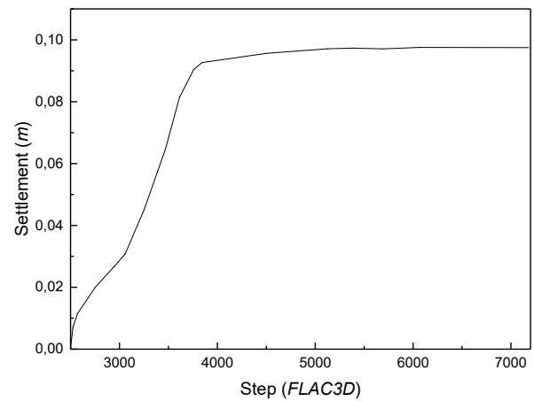
Figure 3 Evolution of vertical displacement of reinforced soil.
