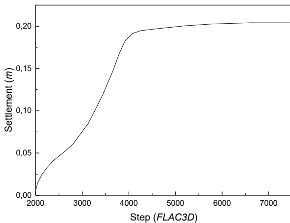
Figure 2 Evolution of vertical displacement of unreinforced soil.
