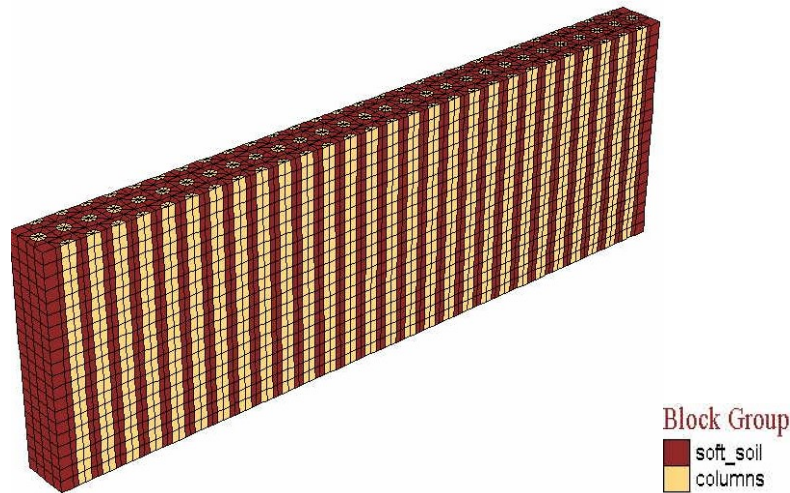
Figure 1 The FLAC 3D numerical modelling of reinforced soil: La Goulette case study, Tunisia
