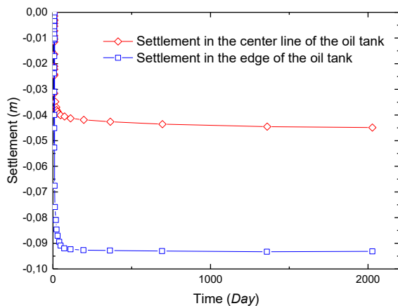
Figure 7 Evolution of the consolidation settlement at the surface of the reinforced soil
