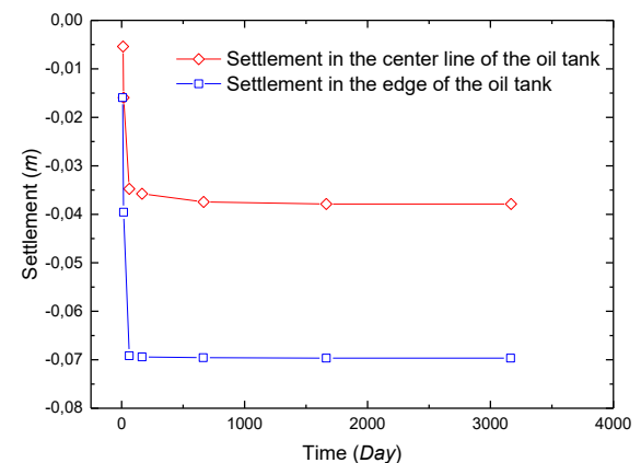
Figure 5 The evolution of the consolidation settlement of the reinforced soil (plane strain condition) Predictions by the HSM (axisymmetric condition)
