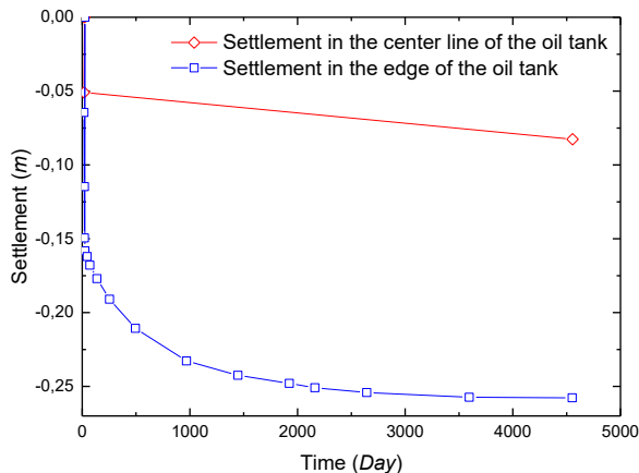
Figure 6 Evolution of the consolidation settlement of the unreinforced soil (axisymmetric condition)
