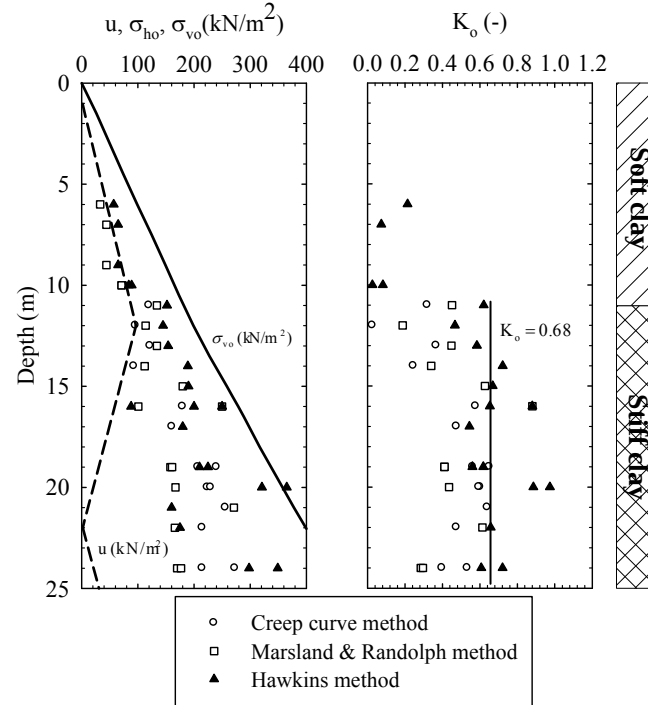
Fig. 9 Total horizontal stresses and coefficient of earth pressure at rest from LLT Tests
