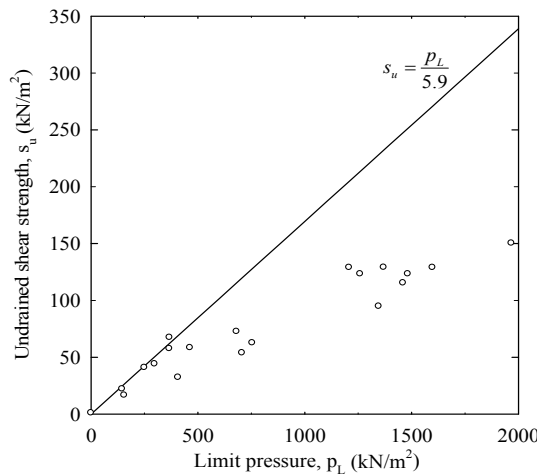
(a) Correlation between undrained shear strength ( s_u ) and limit pressure ( p_L )
