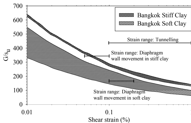
Fig. 6 Variations of G/s_u with shear strain from self-boring pressuremeter tests in Bangkok Soft and Stiff Clays (Modified after Prust et al. , 2005)
