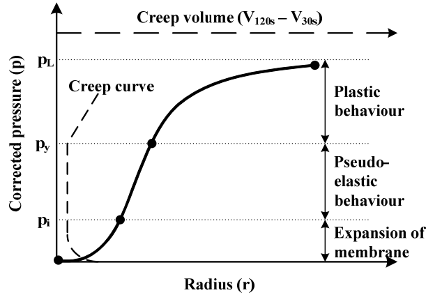
Fig. 7 Typical result for the LLT pressuremeter test
