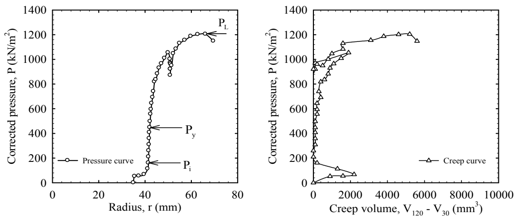
Fig. 8 Pressuremeter test result at Wang Burapha Station in very stiff clay layer at depth of 17 m
