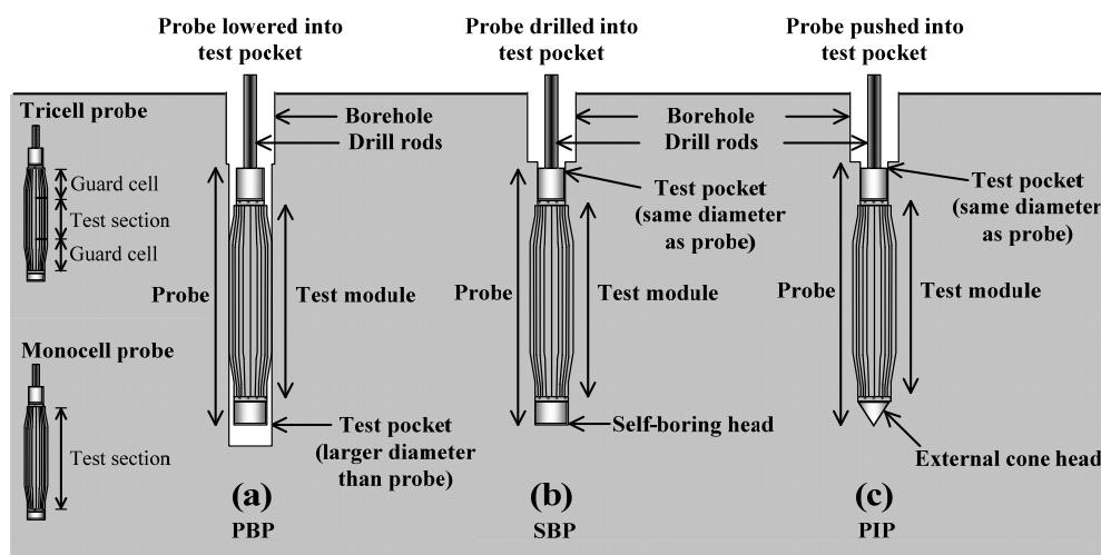
Fig. 3 Pressuremeter probes and test pockets of pre-bored pressuremeter (PBP), self-boring pressuremeter (SBP) and push-in pressuremeter (PIP) (Modified after Clarke, 1995)
