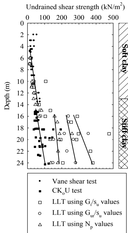
Fig. 10 Comparison of undrained shear strength from field vane shear test, CK_0U triaxial test and LLT tests
