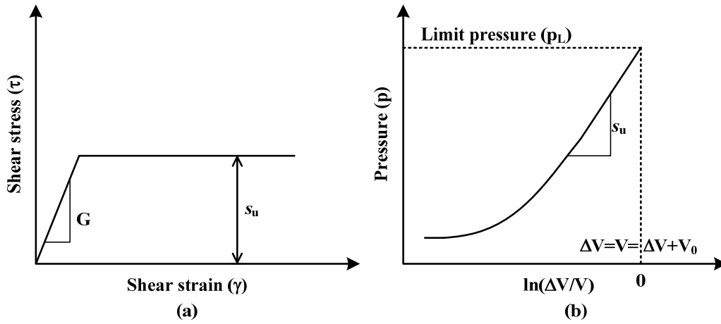
Fig. 5 Undrained shear strength determination from pressuremeter test in clay (Redraw from Schnaid, 2009)
