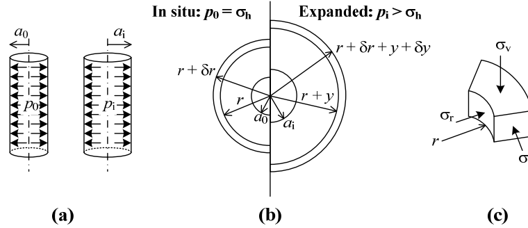
Fig. 4 Definitions used in cavity expansion analysis: (a) expansion of cylindrical cavity; (b) expansion of an element at radius r ; and (c) stress action on an element at radius r (Modified after Clarke 1995)
