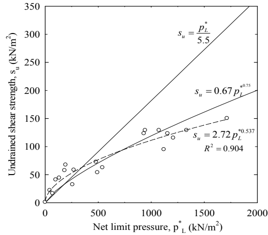
(b) Correlations between undrained shear strength ( s_u ) and net limit pressure ( p_L^* )
