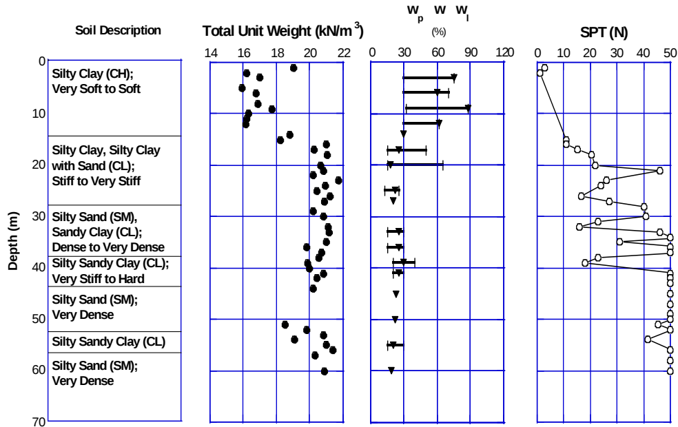
Fig. 2 Soil profile and soil properties for Bangkok MRT Blue Line extension project
