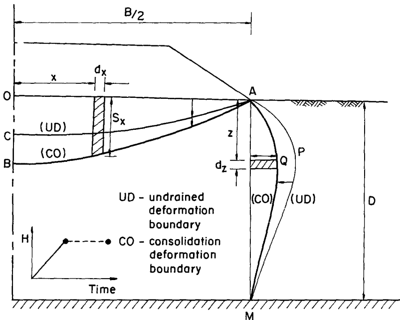
FIG. 3. Deformation Pattern of Embankment Foundation at End of Loading Stage
