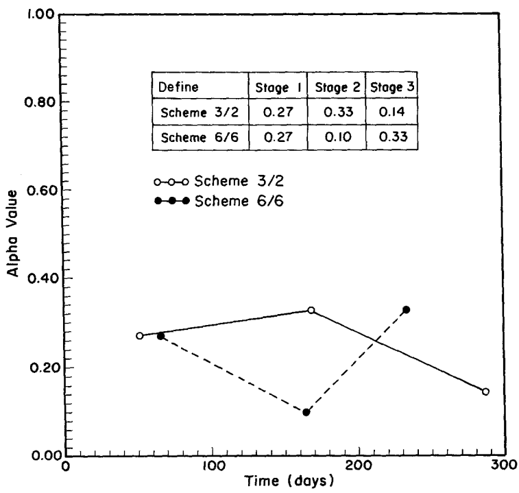
FIG. 5. \alpha -Values for Different Stages of Construction
