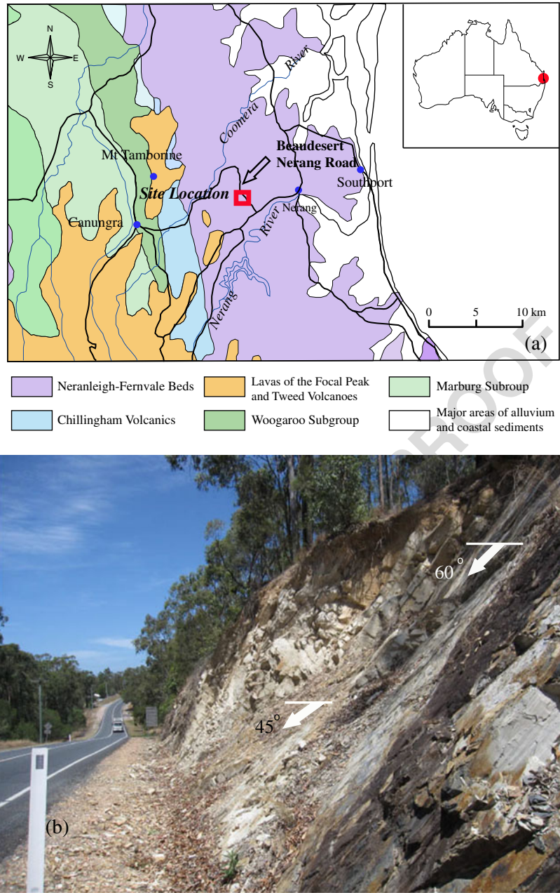
Fig. 3 Geological map (a) and a photo (b) of the study area
