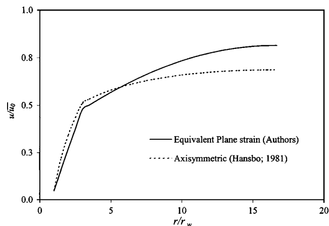
Fig. 4. Normalized excess pore pressure variation with radial (horizontal) direction after 90 days
