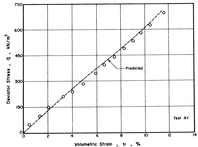
Fig 14. Observed and predicted volumetric strain during drained test with applied stress path of slope (= dq/dp) of 1.5.
