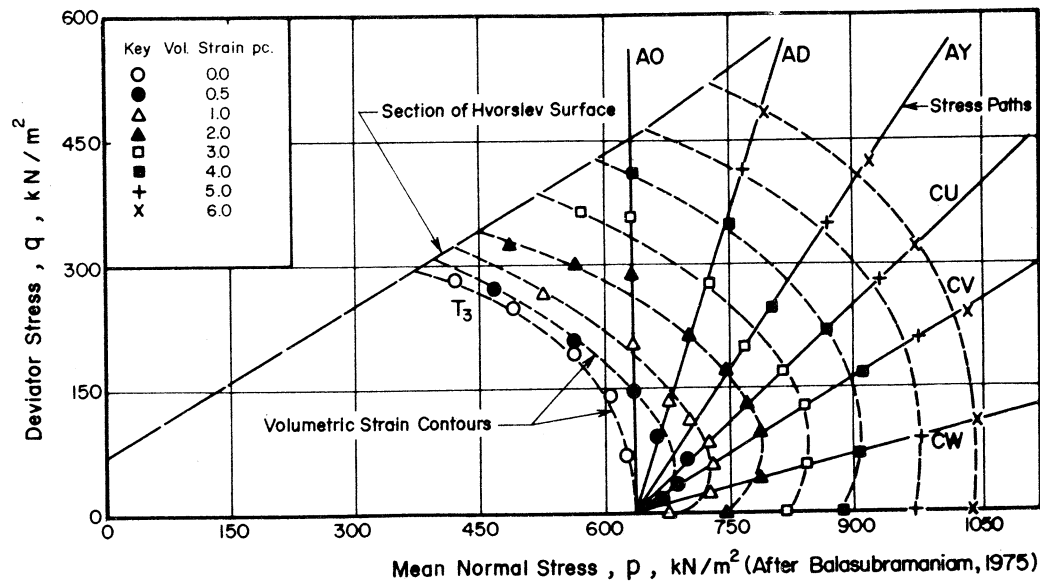
Fig 3. Volumetric strain contours for normally consolidated specimens of Kaolin.
