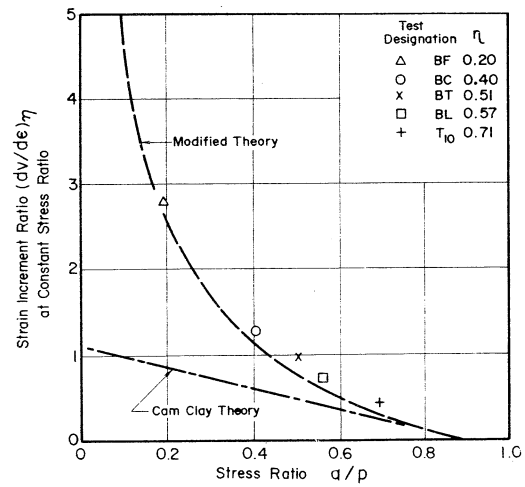
Fig 4. Observed and predicted \left[ \left( \frac{dv}{d\epsilon} \right)_\eta \right] relationship for anisotropic consolidation tests.
