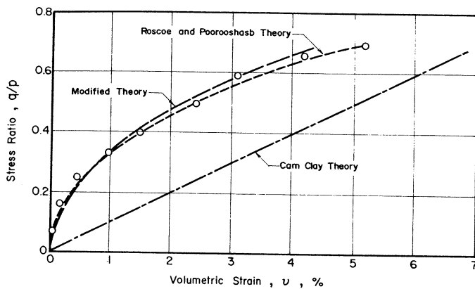
Fig 6. Volumetric strains in constant p test.
