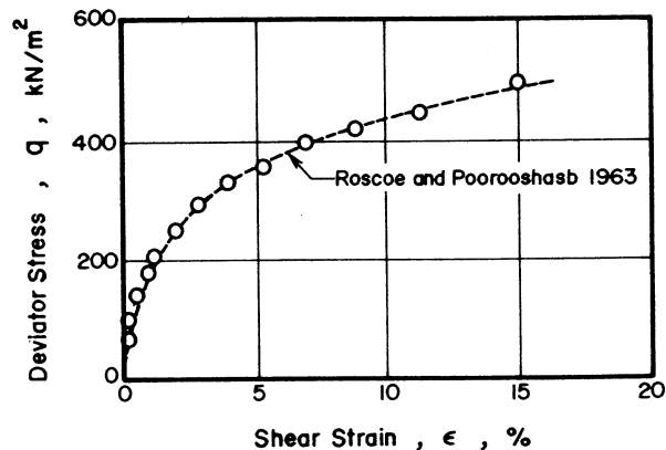
Fig 11. Observed and predicted shear strain for constant p test.
