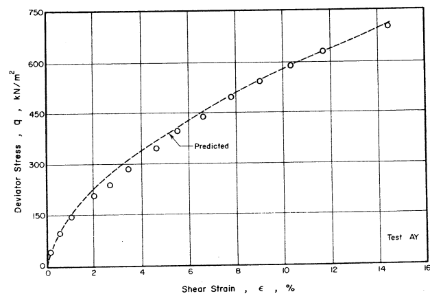
Fig 15. Observed and predicted shear strain during drained test with applied stress path of slope (= dq/dp) of 1.5.
