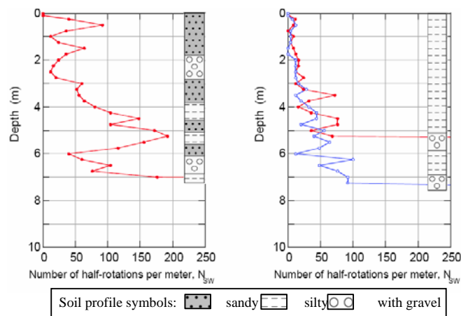
Figure 12. Post-event penetration resistance in Dallington and Avonside measured in SWS tests
